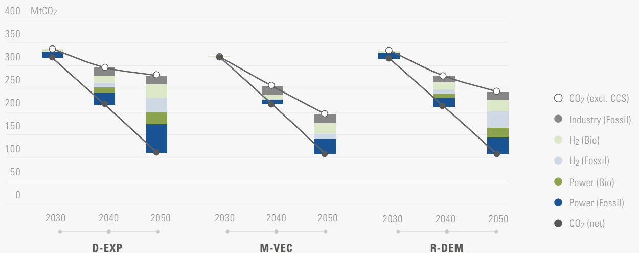
Figure 26. The contribution of CCS to CO 2 mitigation under DDPP scenarios, 2030-2050
