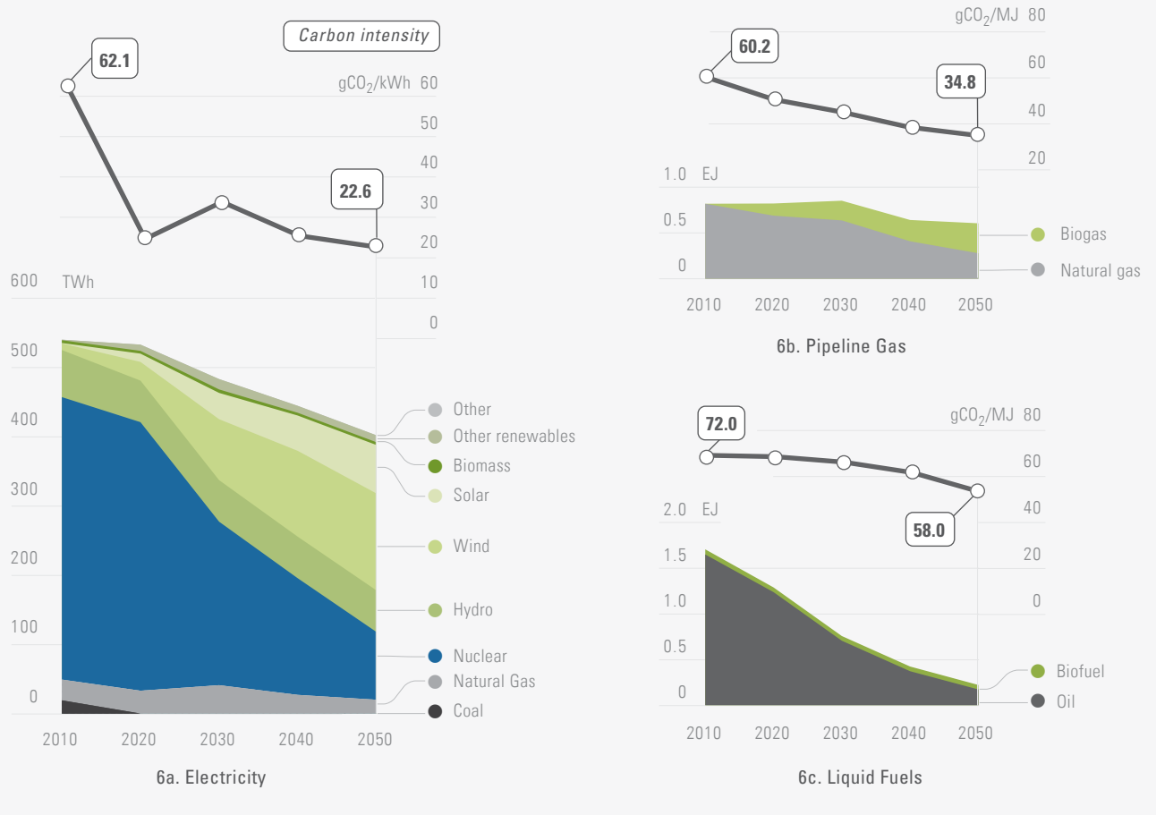
Figure 6. Energy Supply Pathways, by Resource
